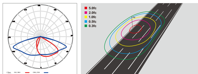
150° (TYPE VS)
