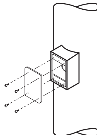
Modification No. 183 Receptacle Outlet Box Only Without Receptacle
